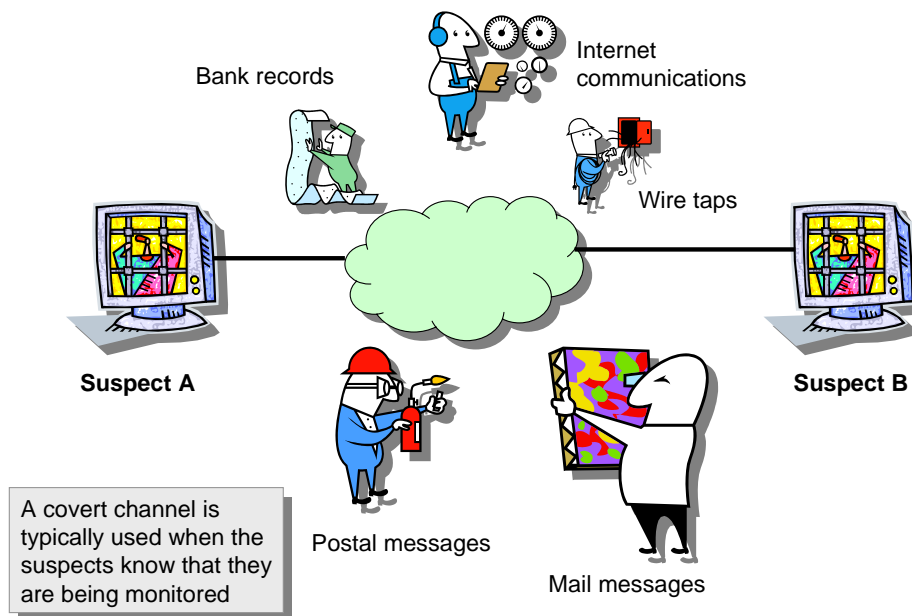
Figure 1: Covert channels
